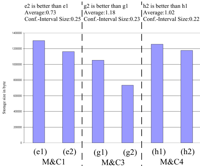
Figure 22. Storage size of sequences
