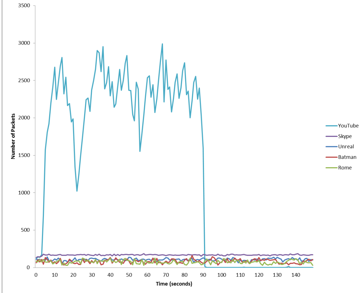
Unreal, Batman, Rome, Skype, and YouTube Upstream: Number of Packets vs Time
