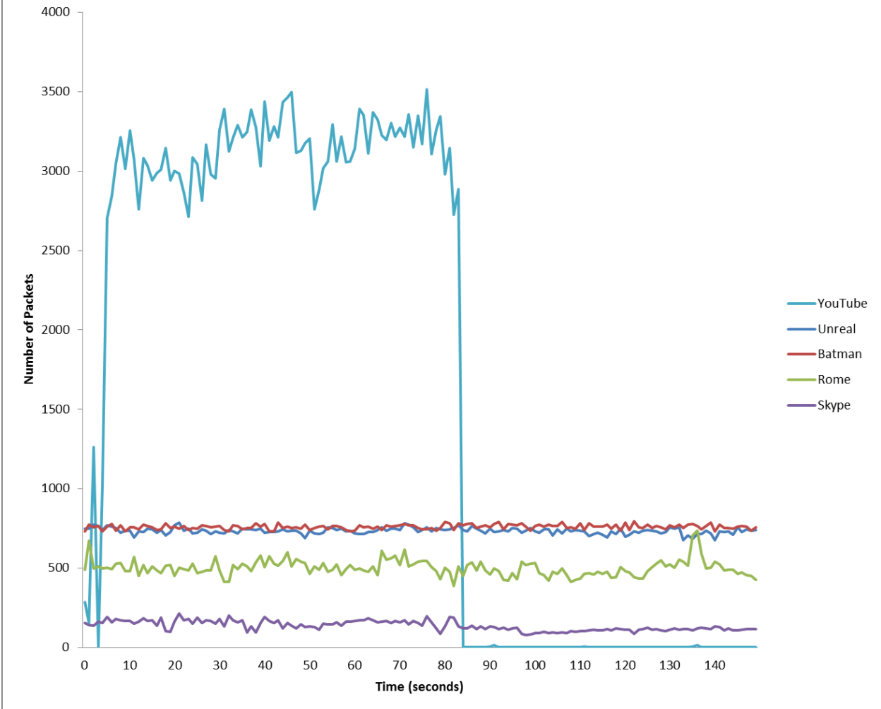
Unreal, Batman, Rome, Skype, and YouTube Downstream: Number of Packets vs Time
