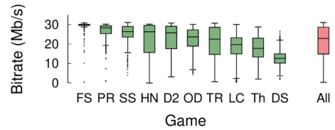
Fig. 2: Downstream game bitrates.
