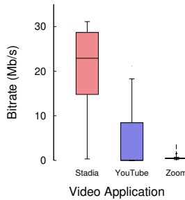
Fig. 8: Downstream bitrates for Stadia, YouTube and Zoom.
