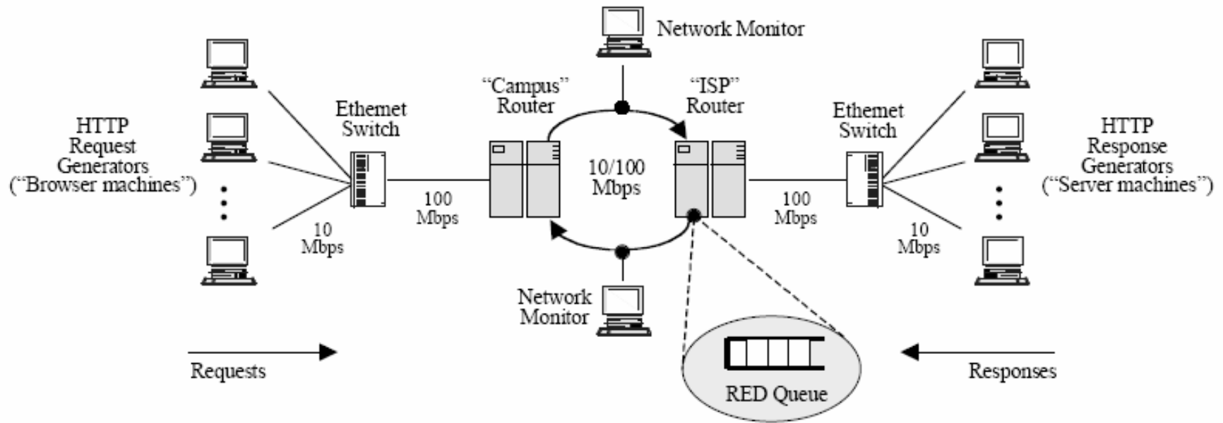
Figure 2: Experimental laboratory network diagram.
