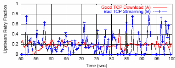
Figure 7: Wireless Layer Retry Fraction
