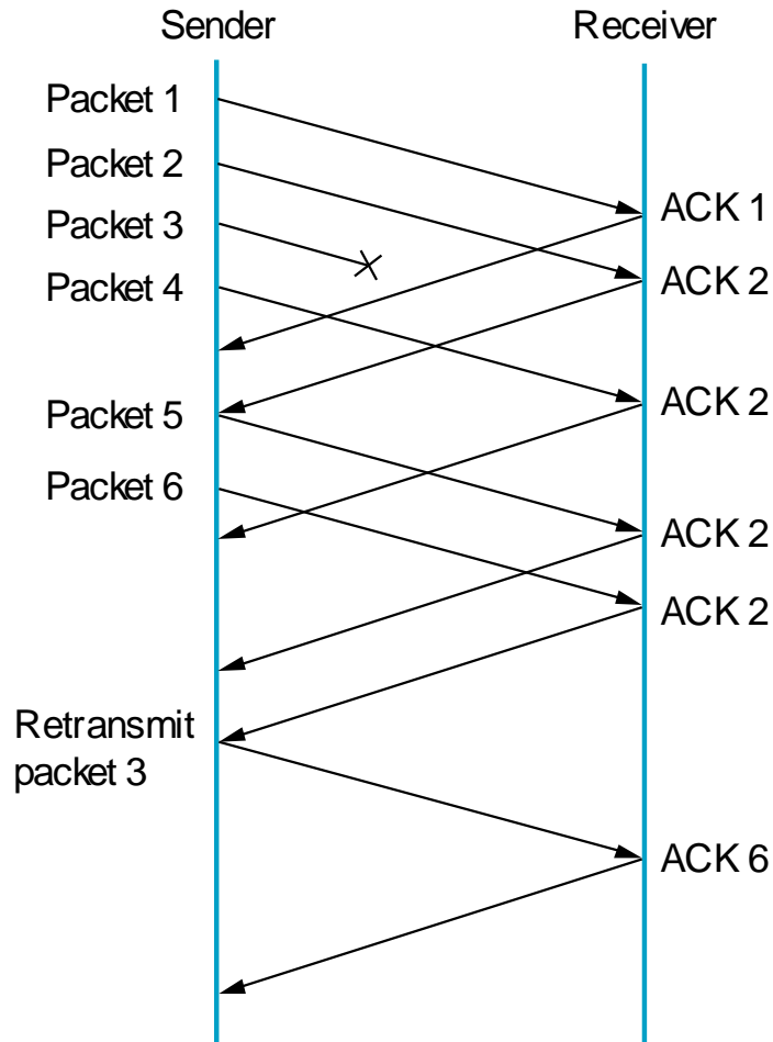
Figure 6.12 Fast Retransmit
